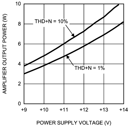
Amplifier Output Power vs Power Supply Voltage R_L = 8\Omega, f = 1kHz
