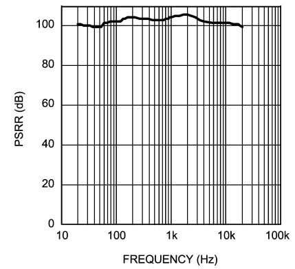
Power Rejection Ratio vs Frequency V_{DD} = 12V, R_L = 8\Omega, \text{Input Referred}
