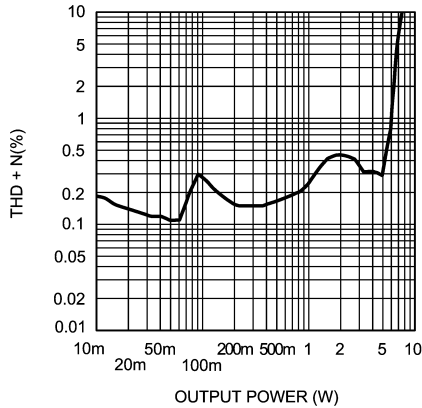
THD+N vs Output Power R_L = 8\Omega, V_{DD} = 12V, f = 1kHz
