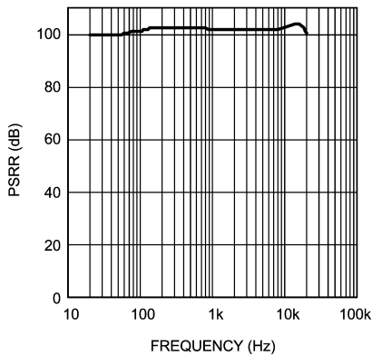
Power Rejection Ratio vs Frequency V_{DD} = 9V, R_L = 8\Omega, \text{Input Referred}
