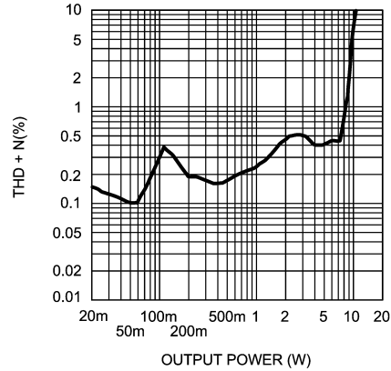
THD+N vs Output Power R_L = 8\Omega, V_{DD} = 14V, f = 1kHz
