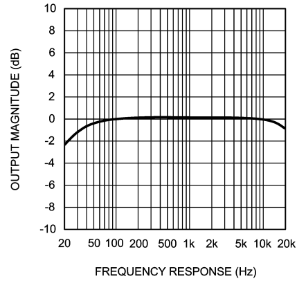
Amplifier Output Magnitude vs Frequency R_L = 8\Omega, V_{DD} = 12V
